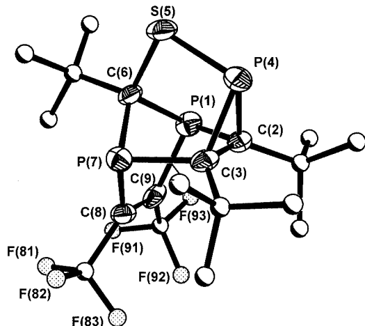
Figure 3. Molecular structure of 18b ; selected bond lengths [Å] and angles [°]; H atoms omitted for clarity, displacement ellipsoids at 50% probability: P(7)–C(8) 1.848(5), P(7)–C(6) 1.872(4), P(7)–C(3) 1.887(4), P(1)–C(9) 1.853(5), P(1)–C(6) 1.866(4), P(1)–C(2) 1.885(4), P(4)–C(3) 1.855(4), P(4)–C(2) 1.865(5), P(4)–S(5) 2.097(2), S(5)–C(6) 1.813(4), C(8)–C(9) 1.341(6), C(3)–C(2) 1.571(6); C(8)–P(7)–C(6) 92.5(2), C(8)–P(7)–C(3) 97.4(2), C(6)–P(7)–C(3) 92.9(2), C(9)–P(1)–C(6) 92.6(2), C(9)–P(1)–C(2) 96.4(2), C(6)–P(1)–C(2) 93.6(2), C(3)–P(4)–C(2) 50.0(2), C(3)–P(4)–S(5) 100.25(14), C(2)–P(4)–S(5) 101.0(2), C(6)–S(5)–P(4) 95.36(14), C(9)–C(8)–P(7) 114.6(3), S(5)–C(6)–P(1) 106.0(2), S(5)–C(6)–P(7) 106.3(2), P(1)–C(6)–P(7) 100.8(2), C(2)–C(3)–P(4) 65.4(2), C(2)–C(3)–P(7) 110.2(3), P(4)–C(3)–P(7) 111.6(2), C(3)–C(2)–P(4) 64.7(2), C(3)–C(2)–P(1) 110.5(3), P(4)–C(2)–P(1) 110.0(2), C(8)–C(9)–P(1) 114.5(3).
