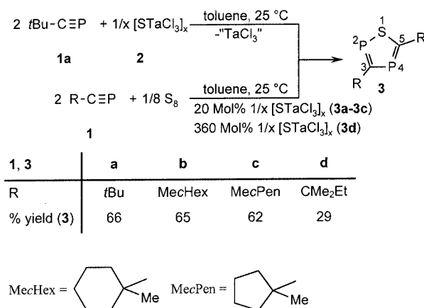
Scheme 1. Synthesis of the 1,2,4-thiadiphospholes 3
