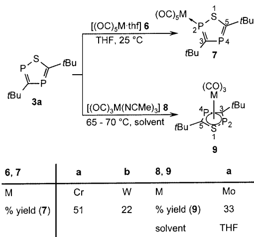
Scheme 3. Group-6 metal complexes of 1,2,4-thiadiphospholes
