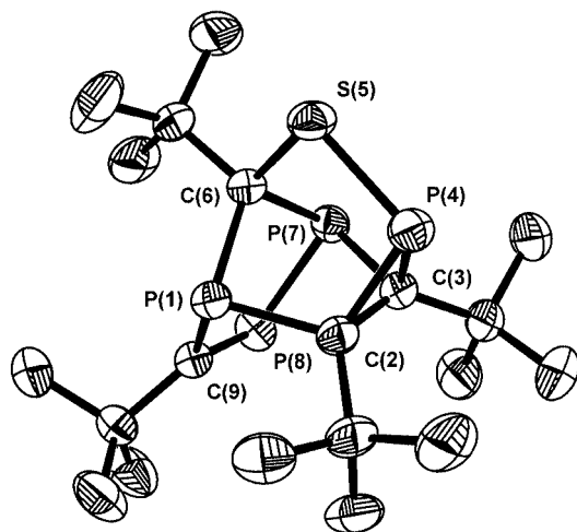
Figure 1. Molecular structure of 11a ; selected bond lengths [Å] and angles [°]; H atoms omitted for clarity, displacement ellipsoids at 50% probability: S(5)–C(6) 1.830(2), S(5)–P(4) 2.0898(9), P(1)–C(9) 1.848(2), P(1)–C(6) 1.880(2), P(1)–C(2) 1.906(2), P(8)–C(9) 1.688(2), P(8)–P(7) 2.2091(7), P(7)–C(6) 1.868(2), P(7)–C(3) 1.877(2), P(4)–C(2) 1.854(2), P(4)–C(3) 1.856(2), C(3)–C(2) 1.566(2), C(6)–S(5)–P(4) 95.82(5), C(9)–P(1)–C(6) 97.97(7), C(9)–P(1)–C(2) 100.06(7), C(6)–P(1)–C(2) 92.51(7), C(9)–P(8)–P(7) 98.33(6), C(6)–P(7)–C(3) 93.59(7), C(6)–P(7)–C(8) 96.81(5), C(3)–P(7)–P(8) 98.26(6), C(2)–P(4)–C(3) 49.94(7), C(2)–P(4)–S(5) 100.41(5), C(3)–P(4)–S(5) 100.46(5), S(5)–C(6)–P(7) 105.33(8), S(5)–C(6)–P(1) 104.61(8), P(7)–C(6)–P(1) 102.15(7), P(8)–C(9)–P(1) 117.54(9), C(2)–C(3)–P(4) 64.95(8), C(2)–C(3)–P(7) 110.81(10), P(4)–C(3)–P(7) 111.04(8), C(3)–C(2)–C(4) 128.91(13), C(3)–C(2)–P(4) 65.10(8), C(3)–C(2)–P(1) 110.98(10), P(4)–C(2)–P(1) 110.75(8).
