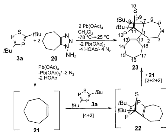
Scheme 6. Reaction between 3a and cycloheptyne ( 21 )
