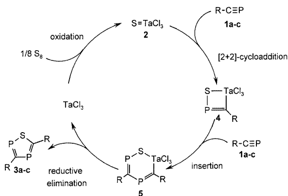
Scheme 2. Proposed reaction mechanism for the catalytic formation of 3a–c
