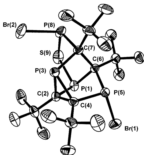
Figure 2. Molecular structure of 14 ; selected bond lengths [Å] and angles [°]: S(9)–P(8) 2.079(2), S(9)–P(1) 2.1382(13), Br(1)–P(5) 2.2871(10), Br(2)–P(8) 2.3129(10), P(1)–C(6) 1.855(3), P(1)–C(2) 1.873(3), P(3)–C(2) 1.841(3), P(3)–C(4) 1.867(3), P(3)–C(7) 1.916(3), P(5)–C(4) 1.822(3), P(5)–C(6) 1.892(3), P(8)–C(7) 1.918(3), C(2)–C(4) 1.569(4), C(6)–C(7) 1.615(4); P(8)–S(9)–P(1) 100.55(5), C(6)–P(1)–C(2) 93.30(12), C(6)–P(1)–S(9) 94.53(10), C(2)–P(1)–S(9) 107.96(10), C(2)–P(3)–C(4) 50.06(12), C(2)–P(3)–C(7) 98.39(13), C(4)–P(3)–C(7) 99.04(12), C(4)–P(5)–C(6) 93.69(12), C(4)–P(5)–Br(1) 100.01(10), C(6)–P(5)–Br(1) 105.92(9), C(7)–P(8)–S(9) 98.31(10), C(7)–P(8)–Br(2) 105.37(9), S(9)–P(8)–Br(2) 100.05(5), C(4)–C(2)–P(3) 65.8(2), C(4)–C(2)–P(1) 108.3(2), P(3)–C(2)–P(1) 109.5(2), C(2)–C(4)–P(5) 112.7(2), C(2)–C(4)–P(3) 64.1(2), P(5)–C(4)–P(3) 107.1(2), C(7)–C(6)–P(1) 105.0(2), C(7)–C(6)–P(5) 102.6(2), P(1)–C(6)–P(5) 99.73(14), C(6)–C(7)–P(3) 104.2(2), C(6)–C(7)–P(8), 108.0(2), P(3)–C(7)–P(8) 106.49(14)
