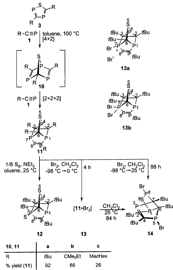
Scheme 4. Synthesis and oxidation of the tetracyclic compound 11
